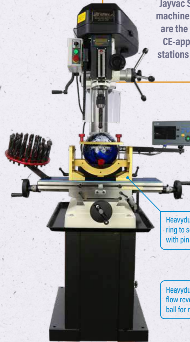
JAYHAWK TRI OVAL SYSTEM 220V-50HZ 250-11-5030-CE
