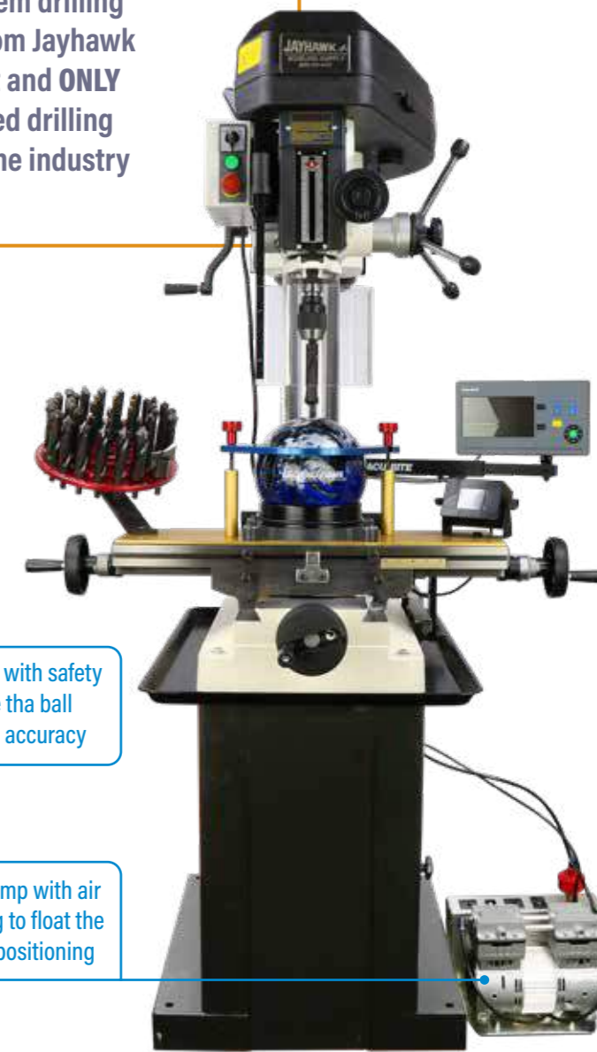
JAYHAWK JAYVAC SYSTEM 220V-50HZ 250-11-5040-CE
